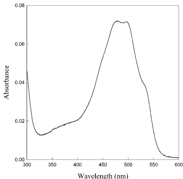
Fig. 2. An absorption spectrum of doxorubicin in water.
